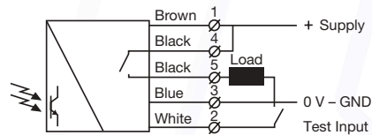
SGR 15 Load as PNP output
