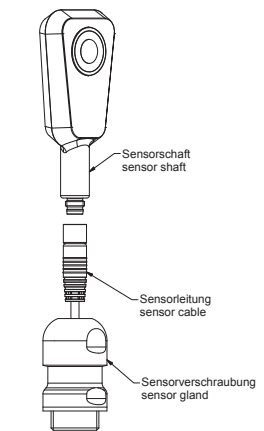
Fig. 4: Mounting of pms sensor with sensor screw connection BF-pms/A1
