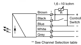
SMT 90X0C Variable range & test input setup
