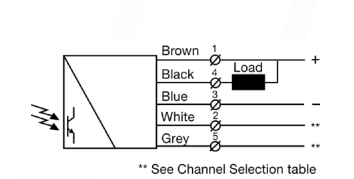
SMR 9XX0 Transistor NPN
