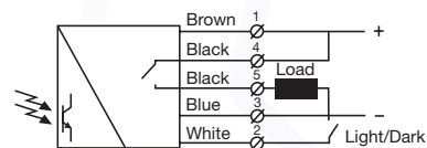
SGR 10 (load as PNP)
