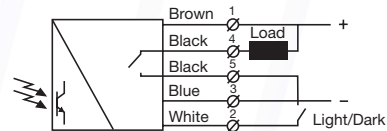
SGR 10 (load as NPN)
